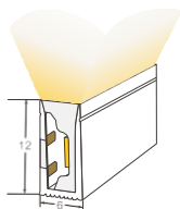
AP-6x12-24V-side bend
